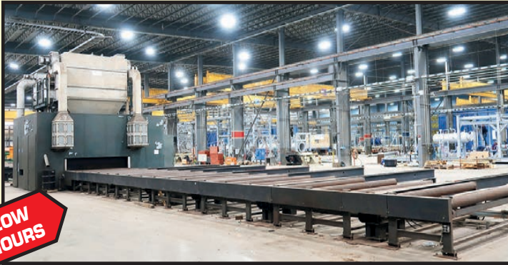
WHEELABRATOR HORIZONTAL PLATE BLASTING LINE
